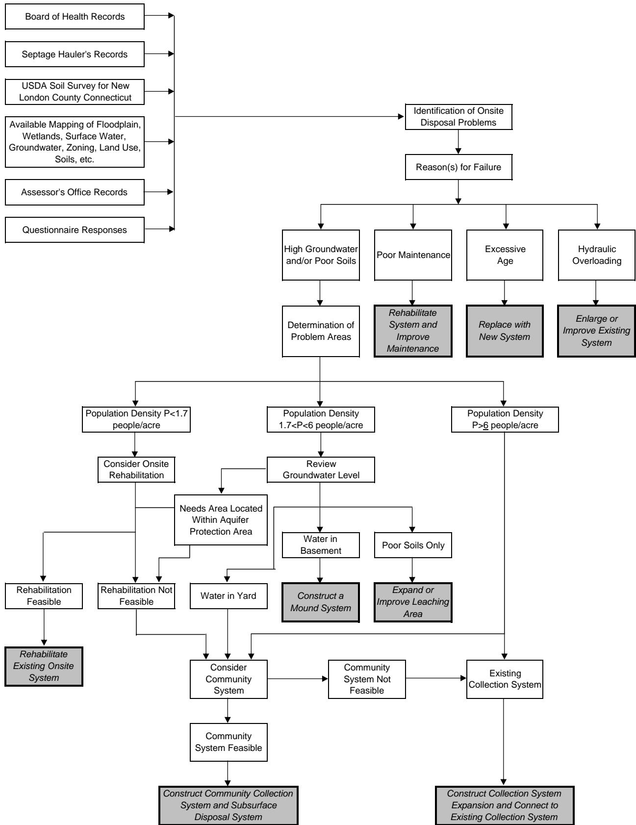
Figure 2-2 Stonington, Connecticut Decision Logic For Wastewater Needs Assessment
